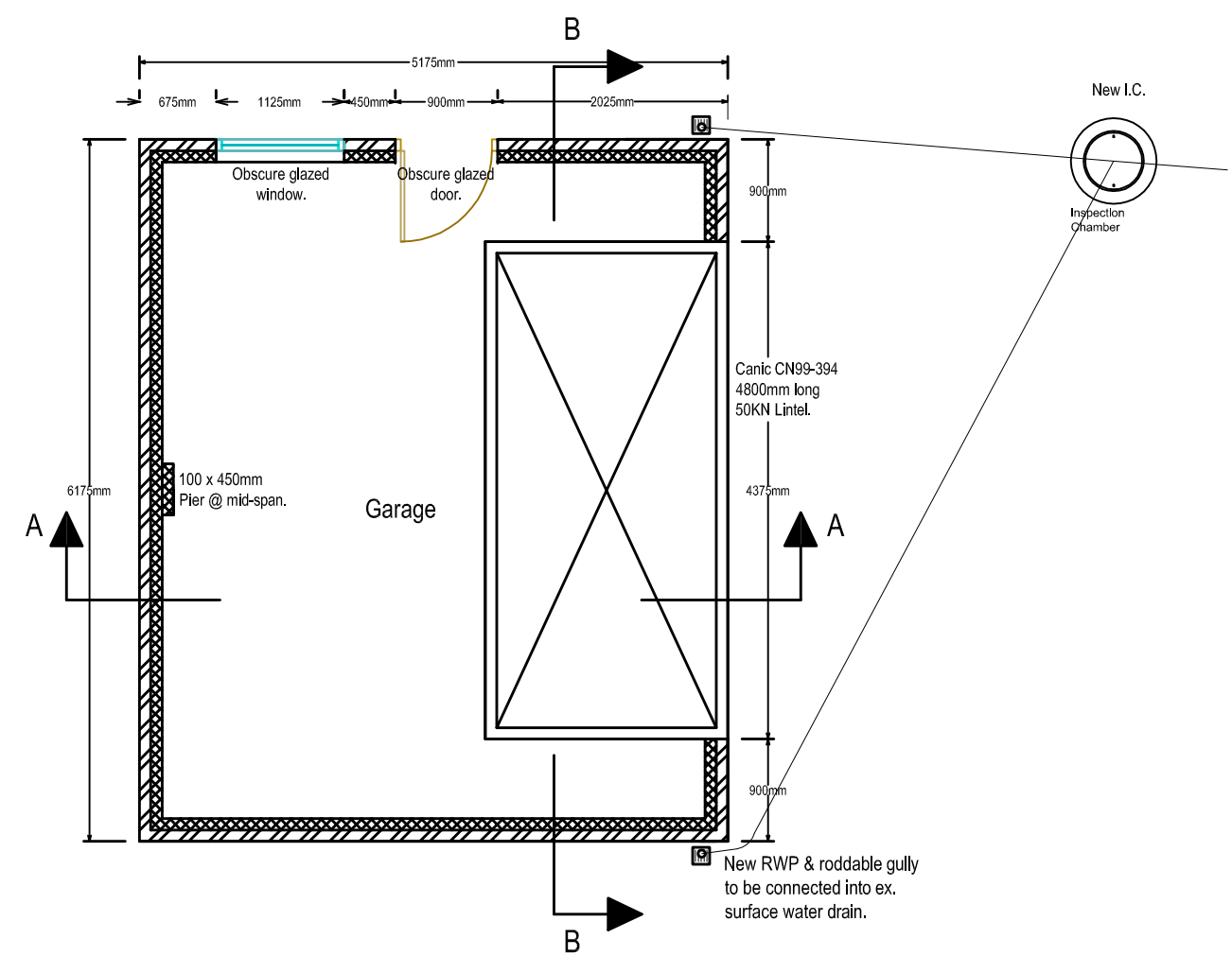
GROUND FLOOR PLAN AS PROPOSED (1:50)
