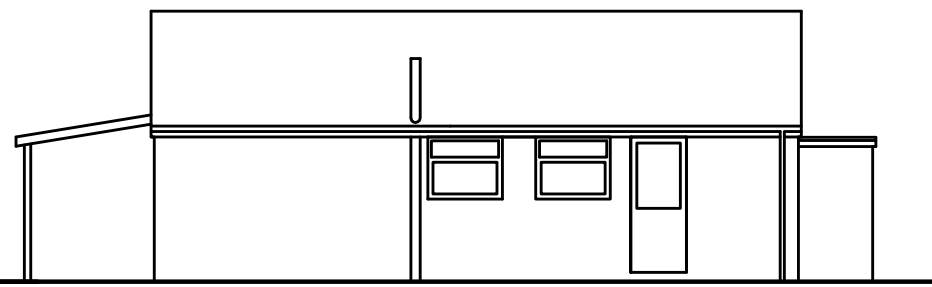
SIDE ELEVATION AS PROPOSED (1:100)
