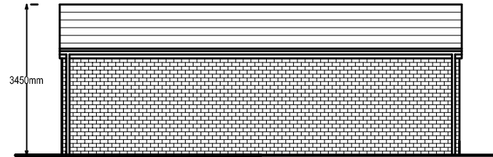
SIDE ELEVATION AS PROPOSED (1:100)
