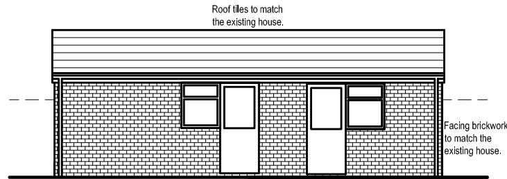
SIDE ELEVATION AS PROPOSED (1:100)
