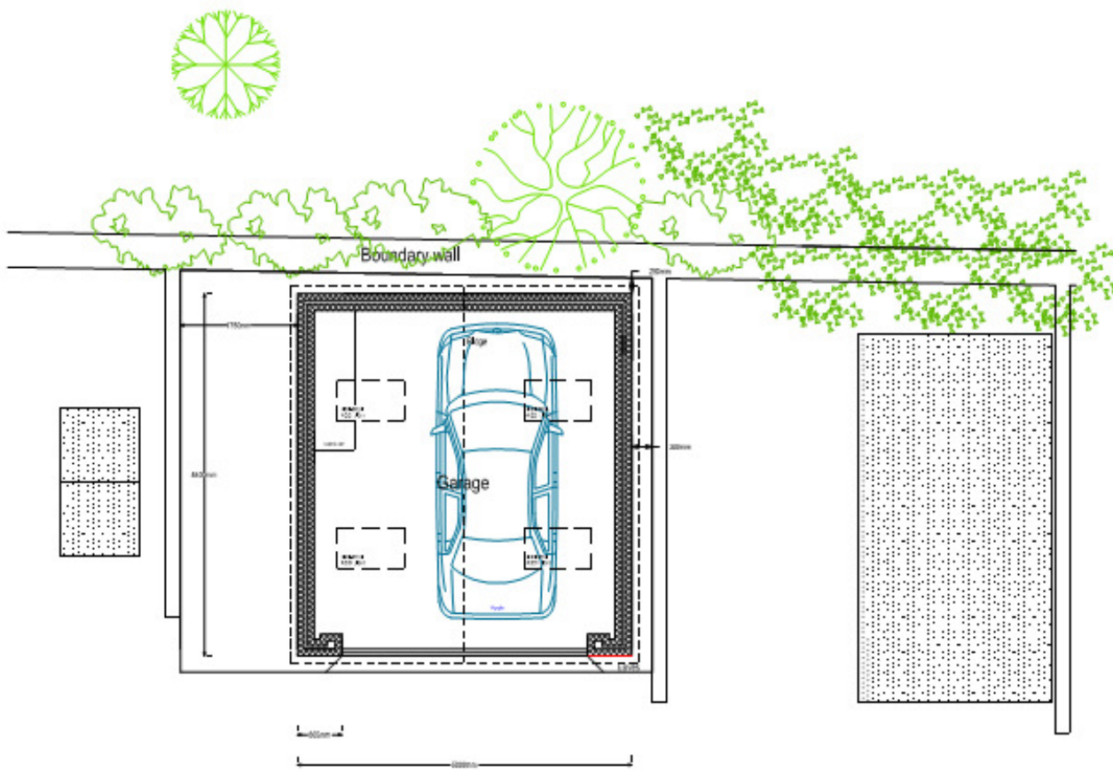
GARAGE PLAN AS PROPOSED (1:50)
