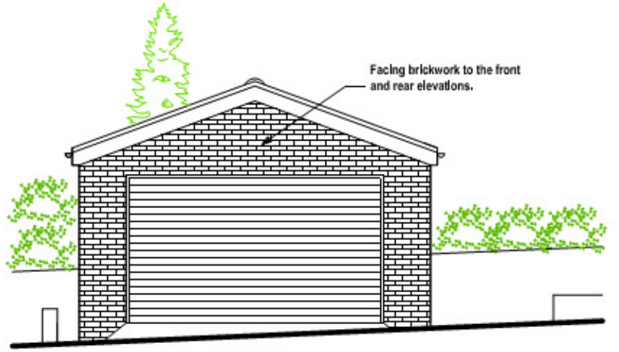
FRONT ELEVATION AS PROPOSED (1:50)
